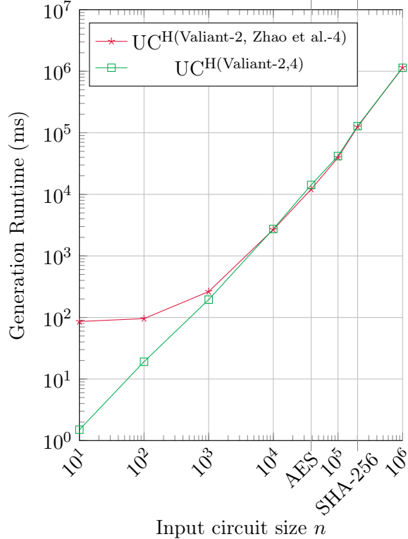
Figure 12: Comparison of the runtime of our hybrid UC implementations using either Valiant’s 2-way and 4-way UCs or Valiant’s 2-way UC with Zhao et al.’s improved block. We note that the runtime of UC^{\text{Zhao et al.-4}} only slightly differs from that of UC^{\text{H(Valiant-2, Zhao et al.-4)}} , and the runtimes of UC^{\text{Valiant-2}} and UC^{\text{Valiant-4}} only slightly differ from that of UC^{\text{H(Valiant-2,4)}} , and therefore we omit them from the figure.
