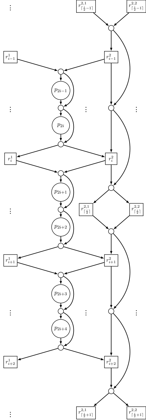
Figure 4: Skeleton built of a chain of body blocks B^{(2)} of Valiant's 2-way EUG U_n^{(2)}(\Gamma_1)
