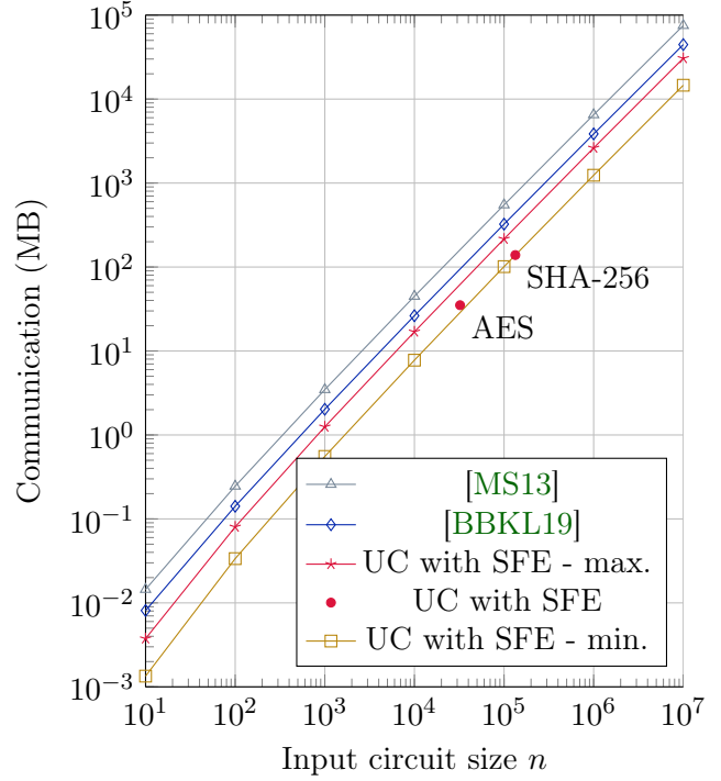
Figure 18: Communication of different PFE protocols in megabytes: UC^H (Valiant-2, Zhao et al.-4) with Yao’s garbled circuits, Mohassel et al.’s OT-based method from [MS13] and its optimized version from [BBKL19].
