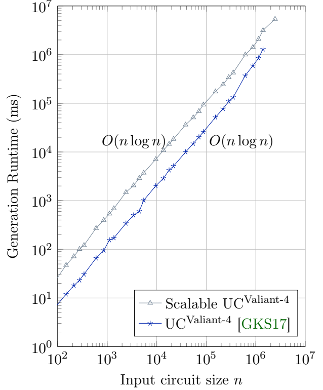
Figure 14: Comparison of the runtime of our per-block and [GKS17]’s UC generations for up to about n = 2\,446\,000 nodes, which fails with [GKS17]’s UC generation and 32 GB of memory.
