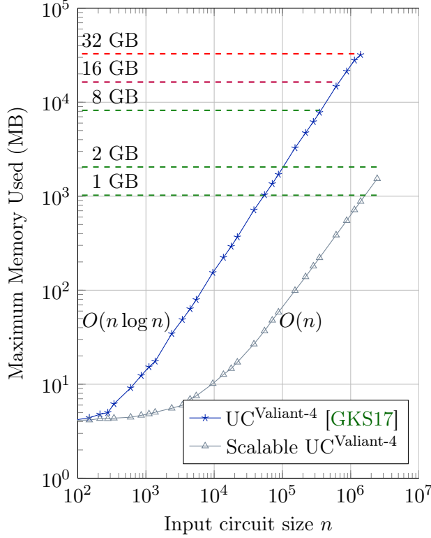
Figure 13: Comparison of the maximum memory used between our per-block and [GKS17]’s UC generation. [GKS17]’s implementation runs out of 32 GB of memory for n > 1\,398\,100 nodes.
