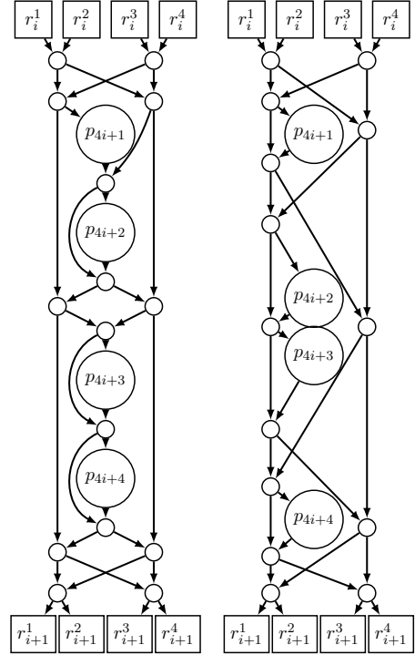
(a) Body block of Valiant [Val76]. (b) Body block of Zhao et al. [ZYZL19].
