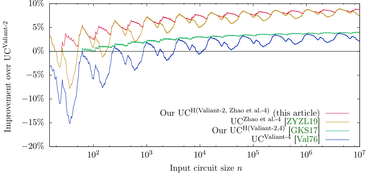
Figure 9: Improvement in size in percentage of our 2/4 hybrid, the 4-way UCs of [Val76, ZYZL19] over Valiant’s 2-way UC for 15 \leq n \leq 10^7 with logarithmic x axis. We note that the different graphs are in the same order as in the legend.
