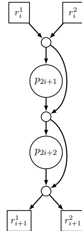
Figure 3: Body block B^{(2)} of Valiant's 2-way EUG U_n^{(2)}(\Gamma_1) [Val76].
