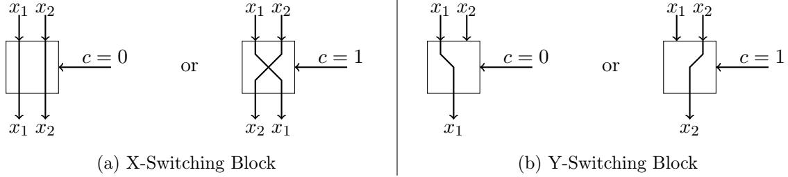
Figure 2: Programmable switching blocks [KS08a].
