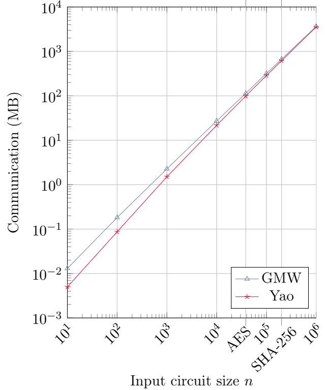
Figure 16: Total communication in megabytes of PFE with the best available UC variant UC^H(\text{Valiant-2, Zhao et al.-4}) .
