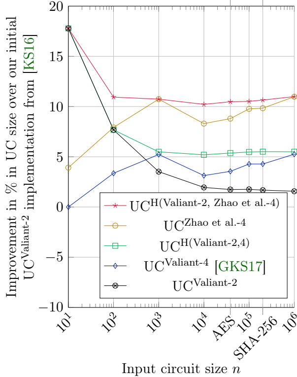
Figure 11: Improvement in percentage of the UC sizes (number of switches) of our UC implementation of Valiant’s 4-way UC^{\text{Valiant-4}} from [GKS17] and our novel implementations including a modular version of Valiant’s 2-way UC^{\text{Valiant-2}} , Zhao et al.’s improved block UC^{\text{Zhao et al.-4}} and hybrid constructions UC^{\text{H(Valiant-2,4)}} and UC^{\text{H(Valiant-2, Zhao et al.-4)}} over our implementation of Valiant’s 2-way UC from [KS16].
