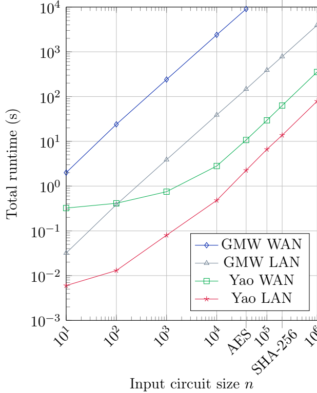
Figure 15: Total runtime in seconds on LAN/WAN of PFE with the best available UC variant UC^H(\text{Valiant-2, Zhao et al.-4}) .
