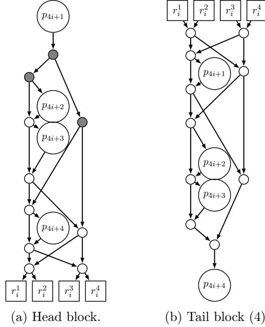
Figure 19: Optimized blocks for Zhao et al.'s 4-way block (Fig. 5b) [ZYZL19].
