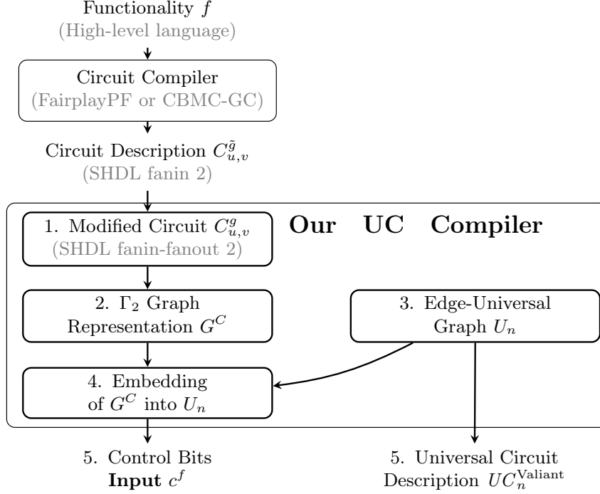
Figure 10: Our universal circuit compiler.
