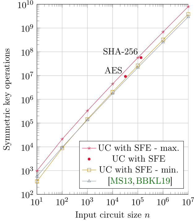
Figure 17: The number of symmetric-key operations of different PFE protocols: Valiant’s UC with Yao’s garbled circuits, Mohassel et al.’s OT-based method from [MS13] and its optimized version from [BBKL19].
