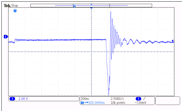
Fig. 6: Voltage trace of VCC glitch
