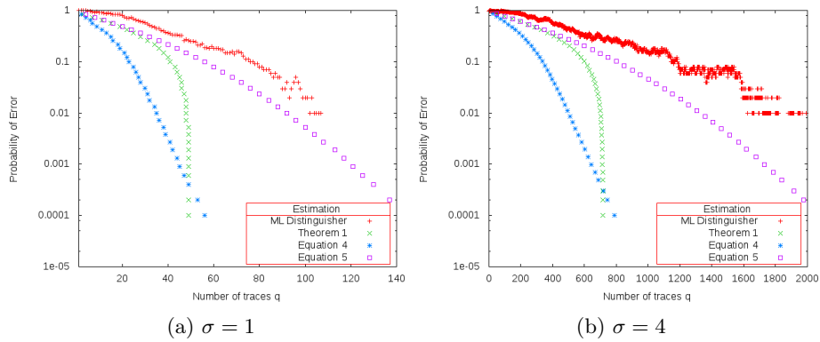
Fig. 5: Error rate for a monobit leakage in a logarithmic scale
