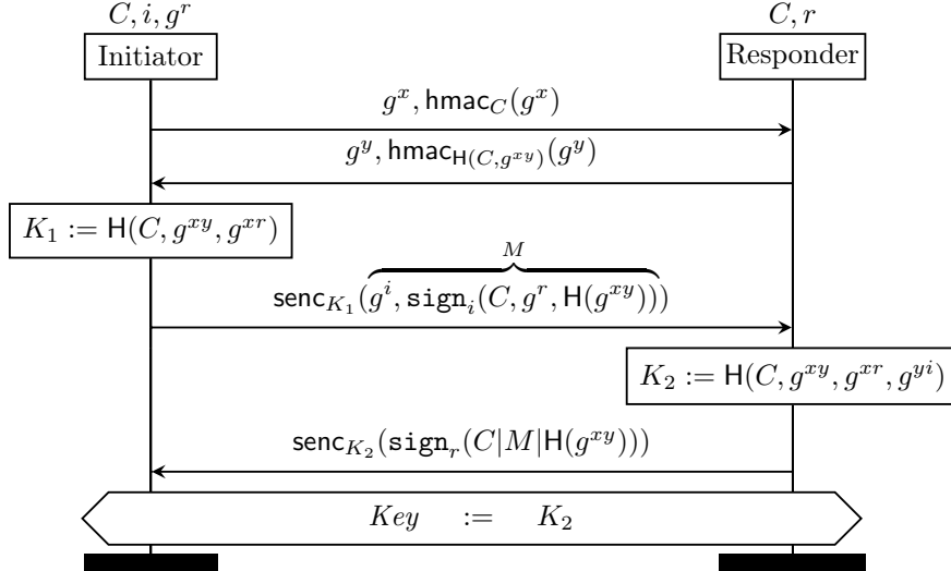
Figure 1: Secure Scuttlebutt’s ‘Secret Handshake’
