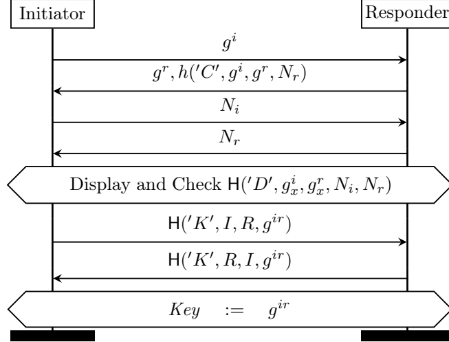
Figure 2: Bluetooth’s Simple Secure Pairing Handshake
