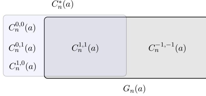
Figure 2: The sets C_n^* and G_n(a)
