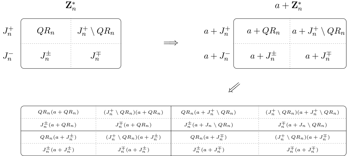
Figure 1: Partitioning the set a + \mathbb{Z}_n^* when n is an RSA modulus
