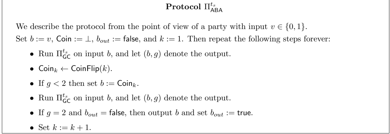
Figure 5: A protocol for Byzantine agreement.
