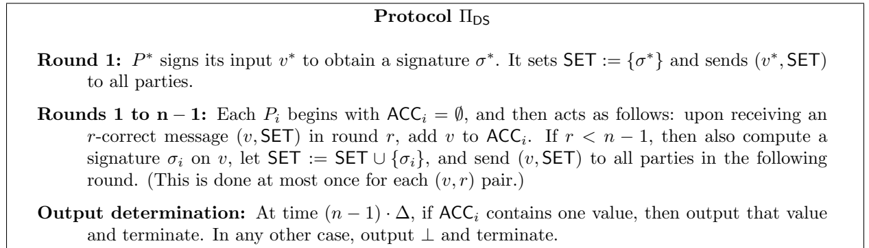
Figure 1: The Dolev-Strong broadcast protocol \Pi_{DS} .
