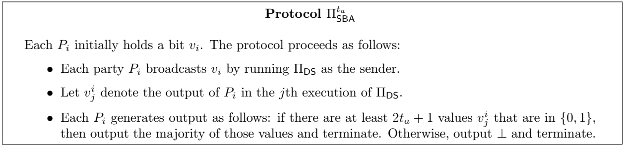
Figure 2: A Byzantine agreement protocol, parameterized by t_a .
