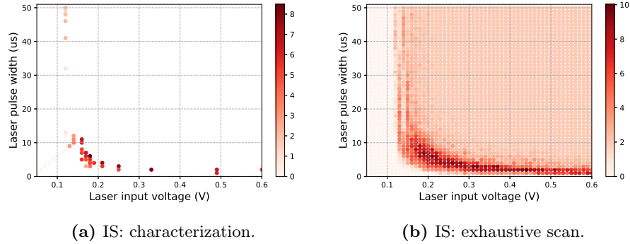
Fig. 11. IS distribution with different fault injection settings for AES encryption.
