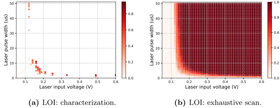
Fig. 9. LOI distribution with different fault injection settings.
