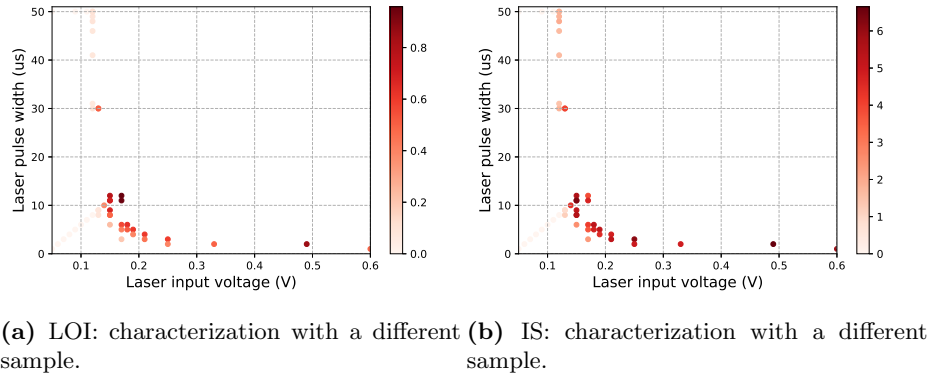
Fig. 12. Characterization results with a different sample targeting AES encryption.
