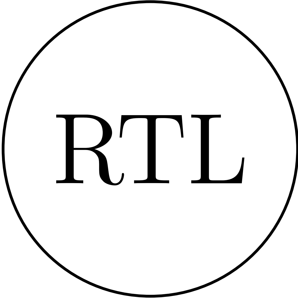
Figure 2: The RaC representation of COFB-like modes
