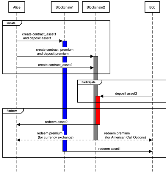
Figure 7: Sequence diagram of our Atomic Swap. For currency exchange-style Atomic Swaps, the premium will go back to Alice if the swap is successful (the left dotted line). For American Call Option-style Atomic Swaps, the premium will go to Bob if the swap is successful (the right dotted line).
