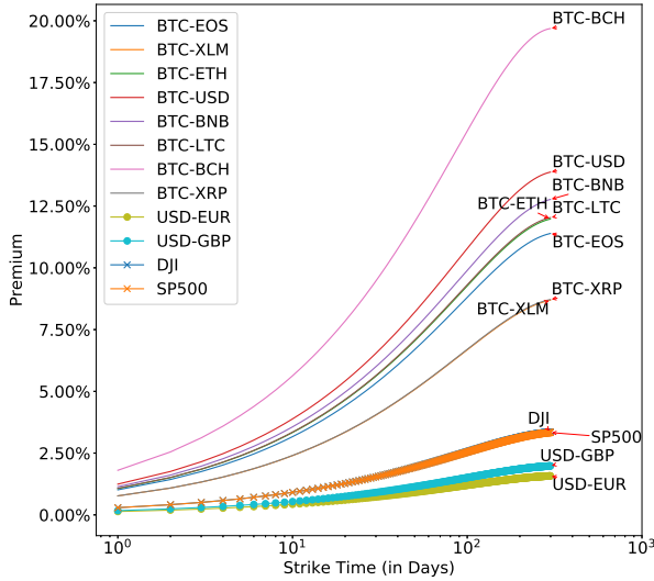
Figure 6: Estimated premium with different strike times for each cryptocurrency pair, stock index and fiat currency pair. Lines with the marker “x” are for stock indices; lines with the marker “o” are for fiat currencies; and lines without marker are for cryptocurrency pairs.
