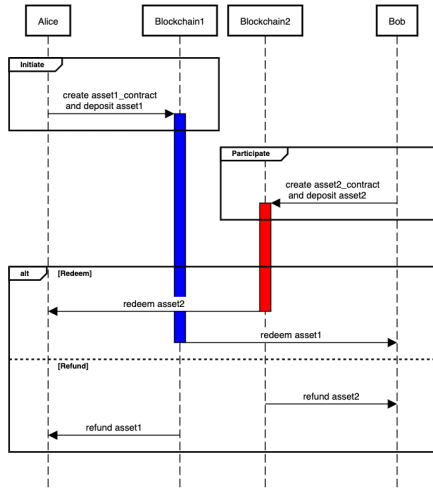
Figure 1: Sequence diagram of Atomic Swap.
