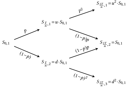
Figure 5: The binomial price tree \mathcal{T} .
