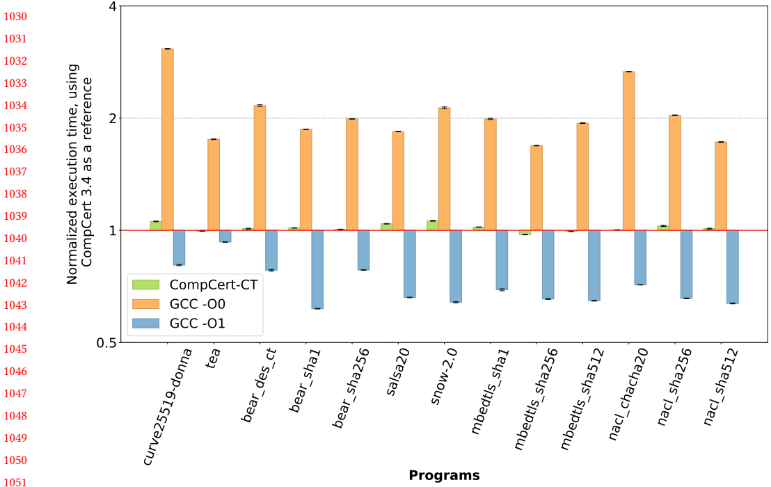
Fig. 10. Execution times of our benchmark. We compare the original CompCert, our modified CompCert, gcc -O0 and gcc -O1. We normalized the measured execution times with the execution time of the original CompCert, which is represented by the red line on the graph. A bar below (resp. above) the red line represents a shorter (resp. longer) execution time. Every tick on the vertical axis represents a factor of two. The error bars represent the 99% confidence intervals of our measurements.
