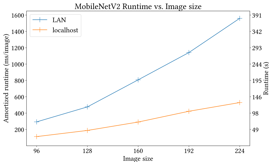
Fig. 1: Runtime vs. Image size of LAN and localhost MobileNetV2 models. See Table 8 for the corresponding accuracies.
