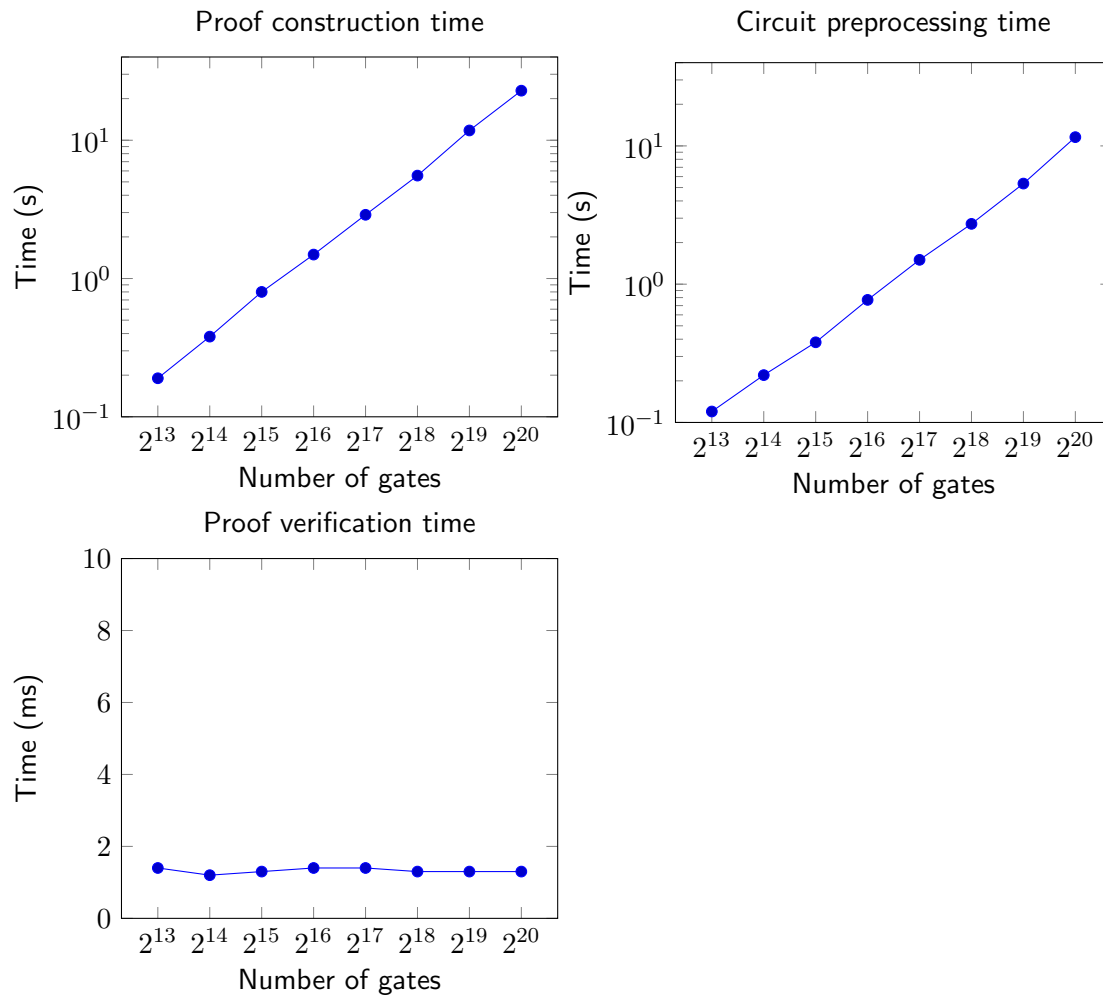
Figure 1: Benchmarks for test *plonk* circuits using the BN254 curve. Does not include witness generation. Tests performed on a Surface pro 6 with 16GB RAM and a core i7-8650U CPU, utilizing all 8 logical/4 physical cores.
