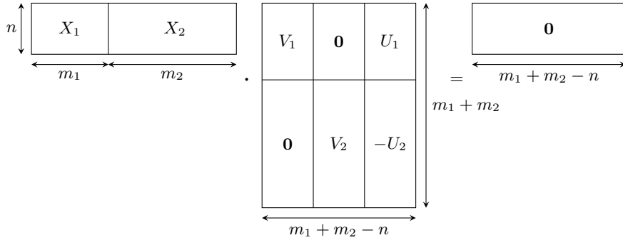
Fig. 2: Given a wide matrix X = [X_1|X_2] \in \mathbb{Z}^{n \times (m_1+m_2)} , we first obtain m_1 + m_2 - n linearly independent short vectors in \Lambda^\perp([X_1|X_2]) . These correspond to the columns [V_1^t|\mathbf{0}]^t and [\mathbf{0}|V_2^t]^t . The n other missing short vectors are obtained via stacking U_i matrices satisfying X_i U_i = I_n , as depicted.
