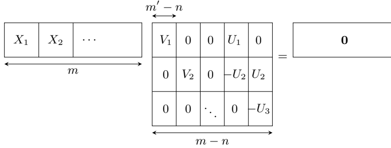
Fig. 1: Technique used in bounding \lambda_{m-n}(\Lambda^\perp(X)) . For each i , the matrix V_i \in \mathbb{Z}^{m' \times m' - n} consists of m' - n short linearly independent vectors orthogonal to X_i , the matrix consisting of the first m' columns of X . The vectors making up V_i are chosen so that they reach the first (m' - n) successive minima of \Lambda^\perp(X_i) . Another n(\frac{m}{m'} - 1) short orthogonal to X vectors are obtained using matrices U_i \in \mathbb{Z}^{m' \times n} that satisfy X_i U_i = I_n and whose columns have small norms.
