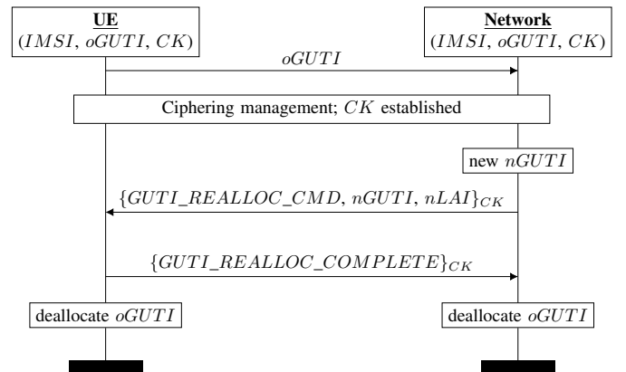
Fig. 5: GUTI Reallocation Procedure.
