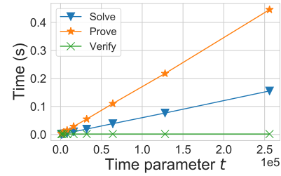
(a) \text{SeqPoW}_{\text{VDF}} + Wes19 [18].
