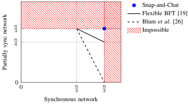
Fig. 3. The flexible BFT protocol can simultaneously support clients who can tolerate f adversaries in a synchronous environment and clients who can tolerate (n-f)/2 adversaries in a partially synchronous environment, for any f between n/3 and n/2 . Thus, there is a tradeoff between the two guarantees. The snap-and-chat protocol achieves (n/2, n/3) , simultaneously optimal. No tradeoff is necessary.
