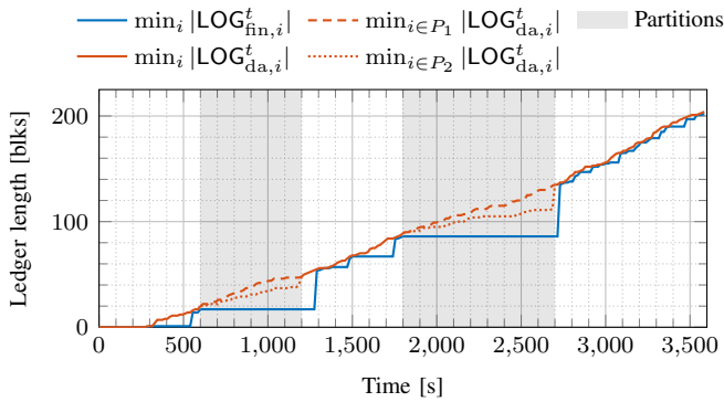
Fig. 10. Under intermittent network partitions, during which honest nodes are split into two parts of 2(n-f)/3 and (n-f)/3 nodes, respectively, finalization of BFT blocks stalls because no 2/3 -quorum is live. The ledgers \text{LOG}_{\text{da}} as seen by the different parts drift apart. Once the network reunites, the honest nodes converge on the longer \text{LOG}_{\text{da}} and \text{LOG}_{\text{fin}} catches up.
