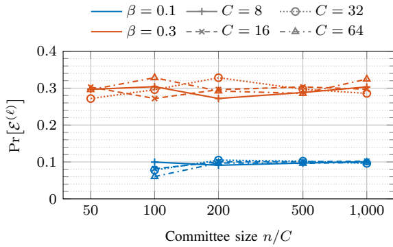
Fig. 12. Monte Carlo estimate of the probability that an adversary who controls \beta fraction of stake can launch the attack in epoch \ell , as a function of number of slots per epoch C and committee size n/C . Observe that \Pr[\mathcal{E}^{(\ell)}] \approx \beta is a good rule of thumb, even for moderate n .
