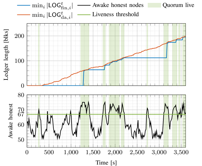
Fig. 9. In a synchronous network where the number of awake honest nodes is modelled by a reflected Brownian motion, \text{LOG}_{\text{da}} grows steadily over time. During intervals in which enough honest nodes are awake there is a 2/3 -quorum to advance \text{LOG}_{\text{fn}} so that it catches up with \text{LOG}_{\text{da}} .
