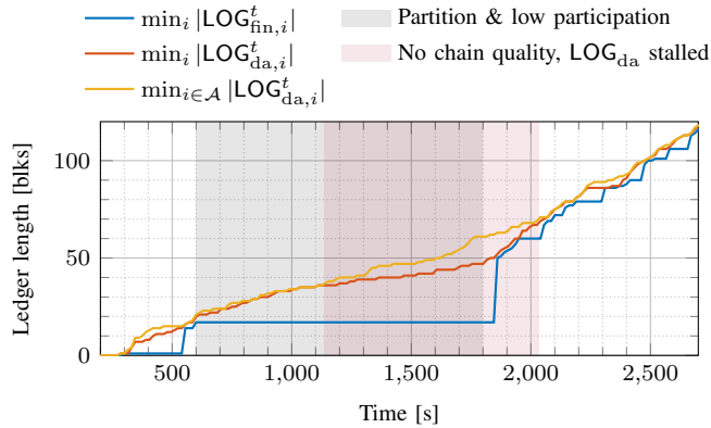
Fig. 10. Under intermittent network partitions, during which honest nodes are split into two parts of 2(n-f)/3 and (n-f)/3 nodes, respectively, finalization of BFT blocks stalls because no 2/3 -quorum is live. The ledgers \text{LOG}_{\text{da}} as seen by the different parts drift apart. Once the network reunites, the honest nodes converge on the longer \text{LOG}_{\text{da}} and \text{LOG}_{\text{fin}} catches up.
