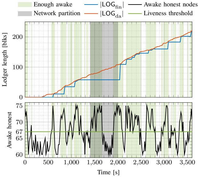
Fig. 2. A simulated run of an example snap-and-chat protocol (combining longest chain and Streamlet [11]) under dynamic participation and network partition. The lengths of the two ledgers are plotted over time. During network partition or when few nodes are awake, the finalized ledger falls behind the available ledger, but catches up after the network heals or when a sufficient number of nodes wake up. See Section IV for details on the simulation setup.
