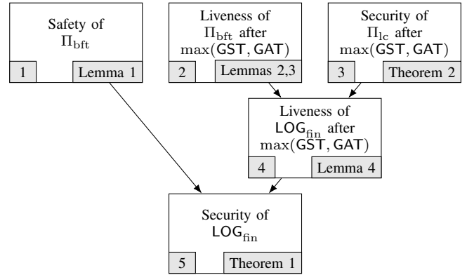
Fig. 7. Dependency of the security of \text{LOG}_{\text{fin}} under (\mathcal{A}_1^*, \mathcal{Z}_1) on the properties of \Pi_{lc} and \Pi_{bft} . Boxes represent the properties and the arrows indicate the implications of these properties. Theorems and lemmas used to validate the properties are displayed at the bottom right corner of each box.
