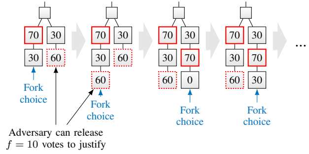
Fig. 13. By releasing withheld Casper FFG votes late, the adversary can force honest validators to adopt a competing chain, due to the modification of the fork choice rule to respect ‘the justified checkpoint of the greatest [depth]’. Over longer periods of time, the adversary forces honest validators to switch back and forth between a ‘left’ and a ‘right’ chain and thus liveness of finalizations is disrupted.
