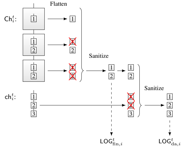
Fig. 6. \text{Ch}_i^t is flattened and sanitized to obtain the finalized ledger \text{LOG}_{\text{fin},i}^t , which is prepended to \text{ch}_i^t and sanitized to form the available ledger \text{LOG}_{\text{da},i}^t .
