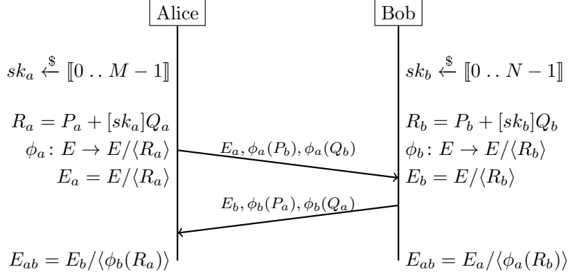
Figure 2: B-SIDH protocol for a prime p such that M|(p+1) and N|(p-1) .
