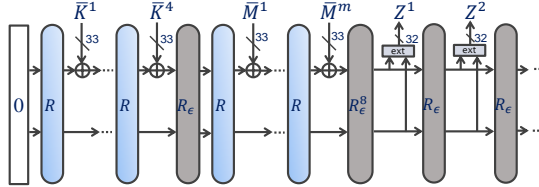
Fig. 2: Subterranean-deck
