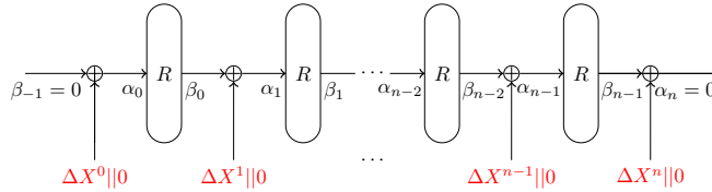
Fig. 5: Differential trails for state collisions
