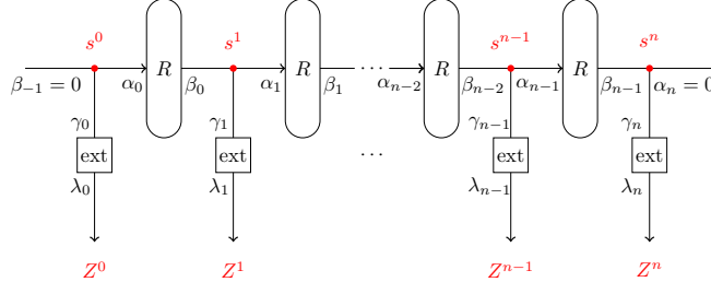
Fig. 4: Linear trails for keystream bias evaluation
