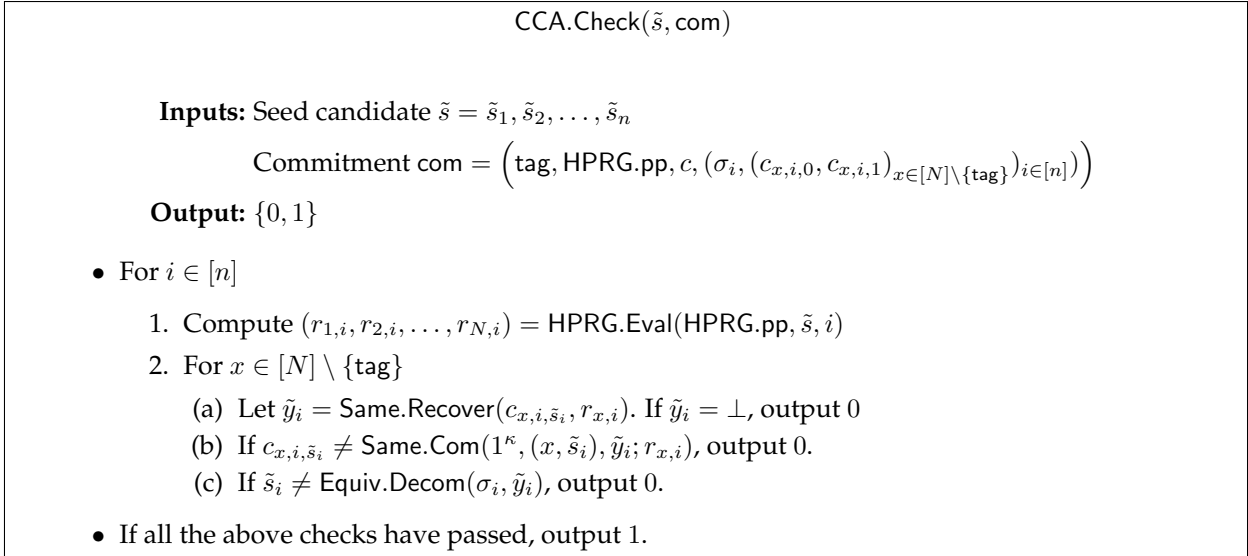
Figure 4: Routine CCA.Check
