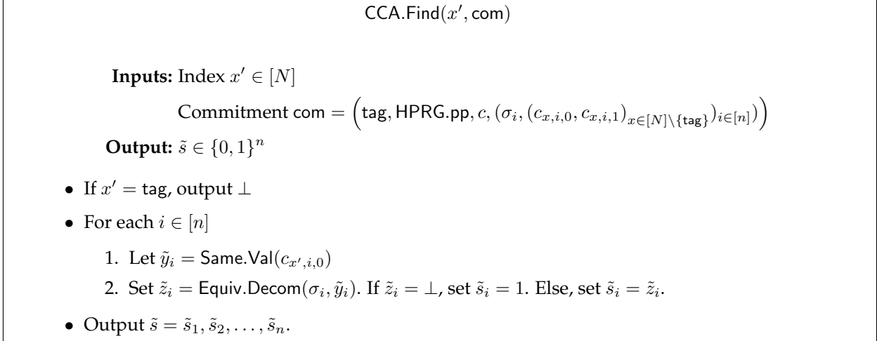
Figure 3: Routine CCA.Find
