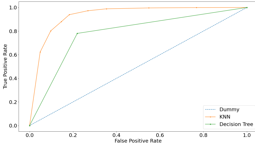
Fig. 8 ROC curve for TWINE (Round 9) experiment ( AUROC_{KNN} = 0.934 , AUROC_{DT} = 0.781 )
