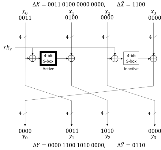
Fig. 1 1 round of a 4-branch GFS with 4-bit S-box
