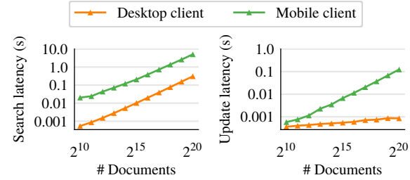
Figure 9: Latency for mobile client and desktop client. Both plots use a logarithmic scale on both axes.
