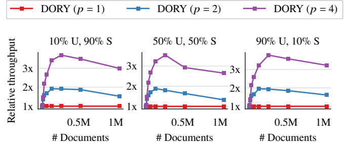
Figure 11: Effect of parallelism ( p denotes the degree of parallelism) on throughput for different workloads (U indicates updates, S indicates searches).
