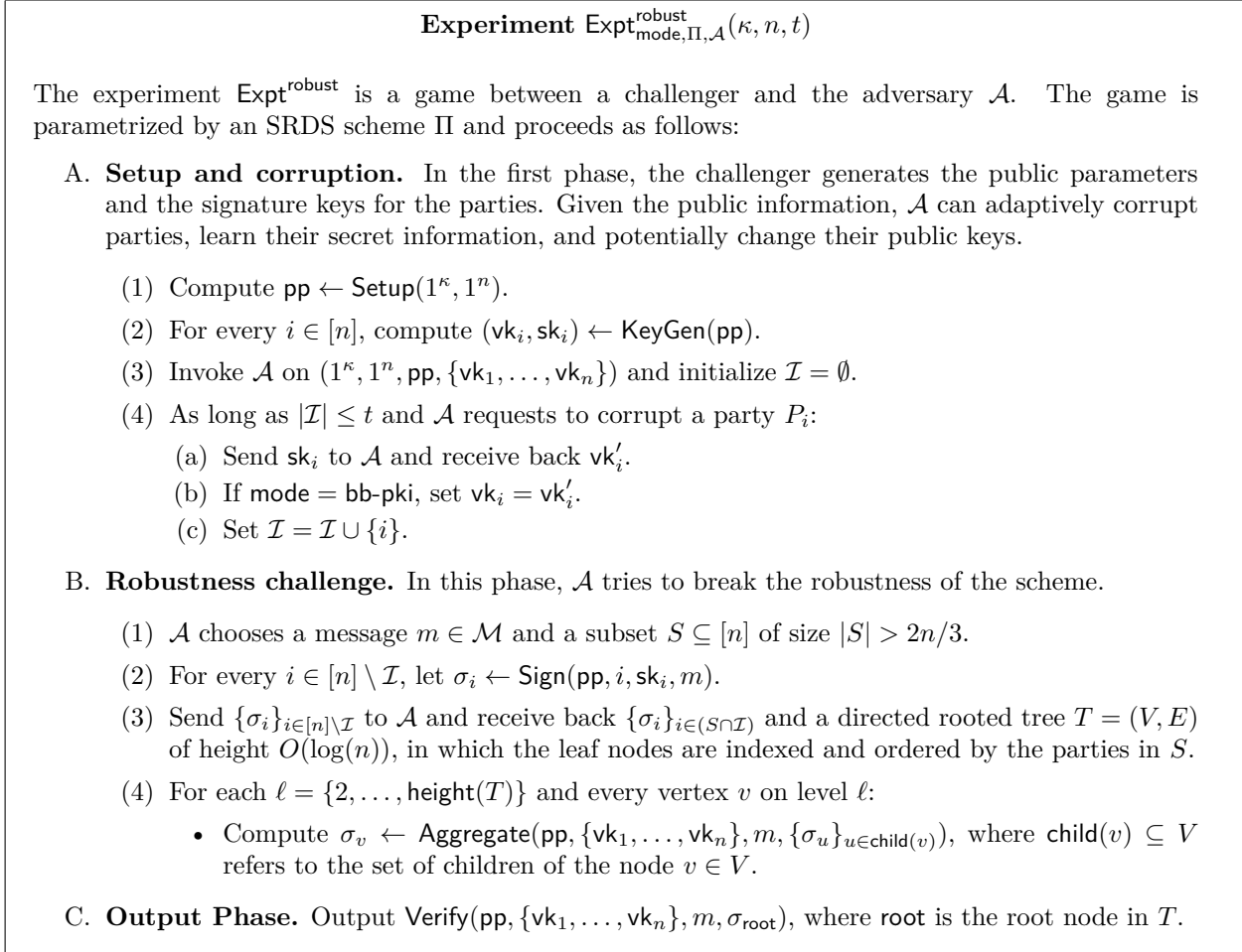
Figure 2: Robustness experiment for SRDS
