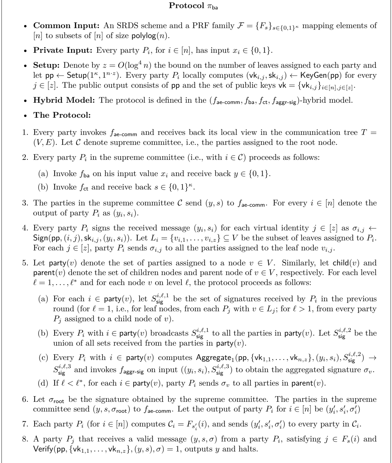
Figure 6: Byzantine agreement with balanced polylog communication
