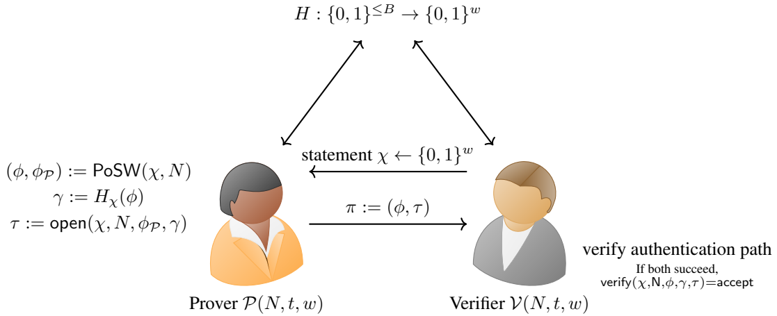
Figure 3: Non-interactive PoSW.
