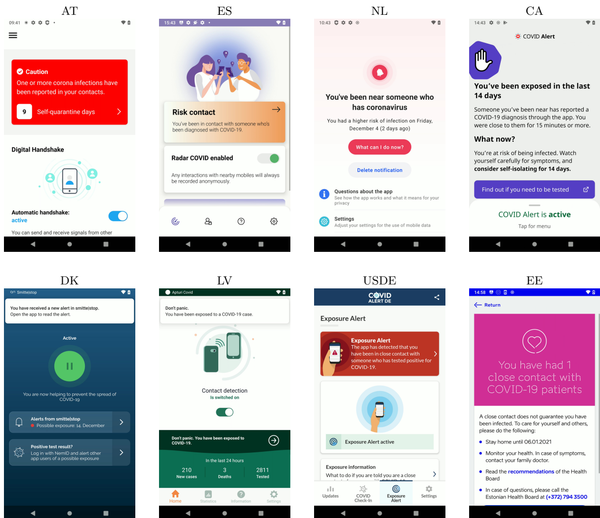
Fig. 9. Screen Captures of More GAEN-Based Apps Raising an Alert
