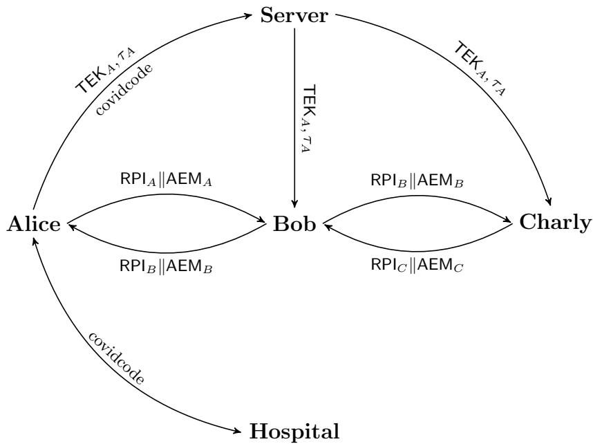
Fig. 3. Exposure Notification Infrastructure
