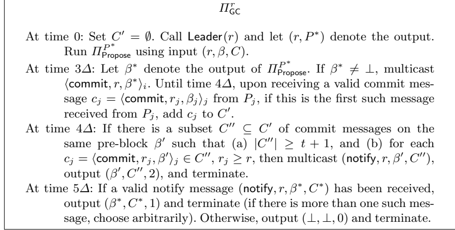
Fig. 8. A graded consensus protocol from the perspective of party P_i with input (r, \beta, C) .
