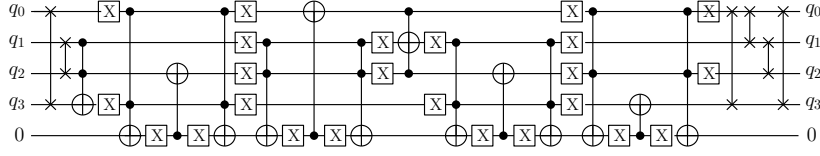
Fig. 7: SATURNIN-256 S-box \sigma_1 .
