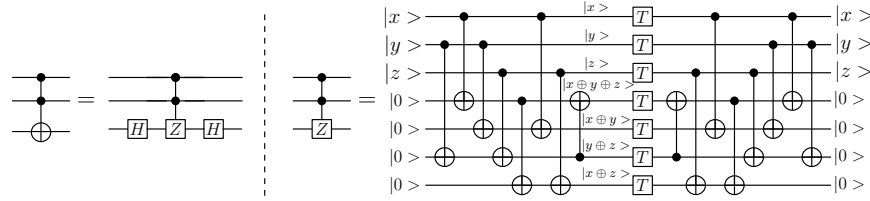
Fig. 2: T -depth 1 representation of the Toffoli gate [15]
