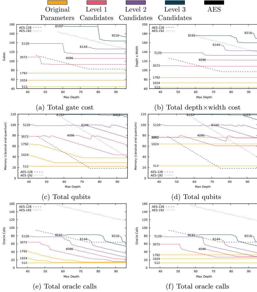
Figure 1: Costs of the quantum collimation sieve attack under various hardware limits. Coloured solid lines are the costs of the collimation sieve at primes of bit lengths from 512 to 9216; dotted lines are the cost of key search on AES, from [21], with the same memory limits and overhead as our analysis. All figures are logarithmic in base 2. Plots on the left are parameterized to minimize gate cost, plots on the right to minimize DW -cost. Larger primes achieving lower depth (e.g., 5120 vs. 4096) is due to increased memory limits.
