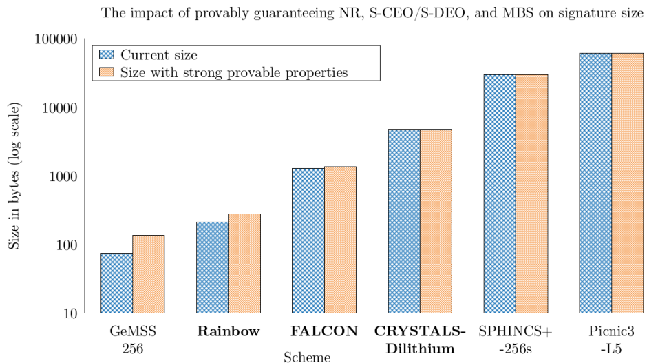
Figure 7: Provably achieving security properties beyond unforgeability for the NIST round 3 candidates: for candidates that do not provably offer these properties yet, our BUFF transformation slightly increases signature size. Since the additional size is constant (64 bytes), the largest relative increase occurs for the smallest signature size (e.g. GeMSS256 goes from 72 to 136 bytes); however, this not even impacts the relative ordering of candidates based on signature size. Since the BUFF transformation involves only a single hash, the additional computational cost is in all cases negligible compared to the signature generation and verification.
