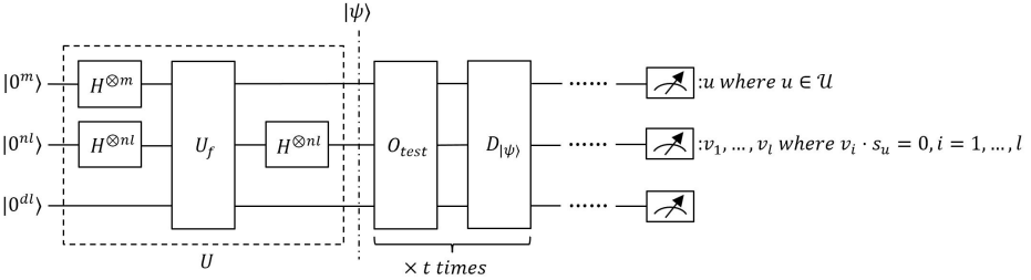
Fig. 16. The quantum circuit of Grover-meet-Simon algorithm.
