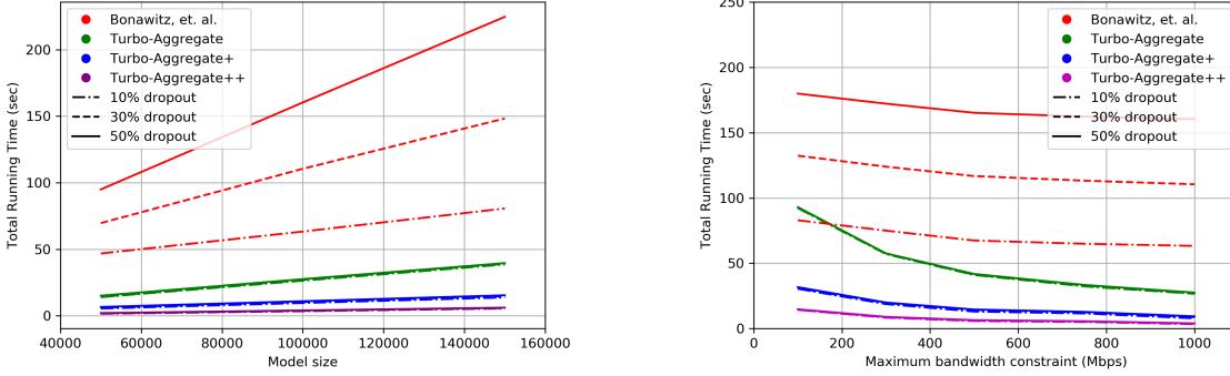
(a) Total running time of Turbo-Aggregate versus the benchmark protocol from [3] as the model size increases, for various user dropout rates.
