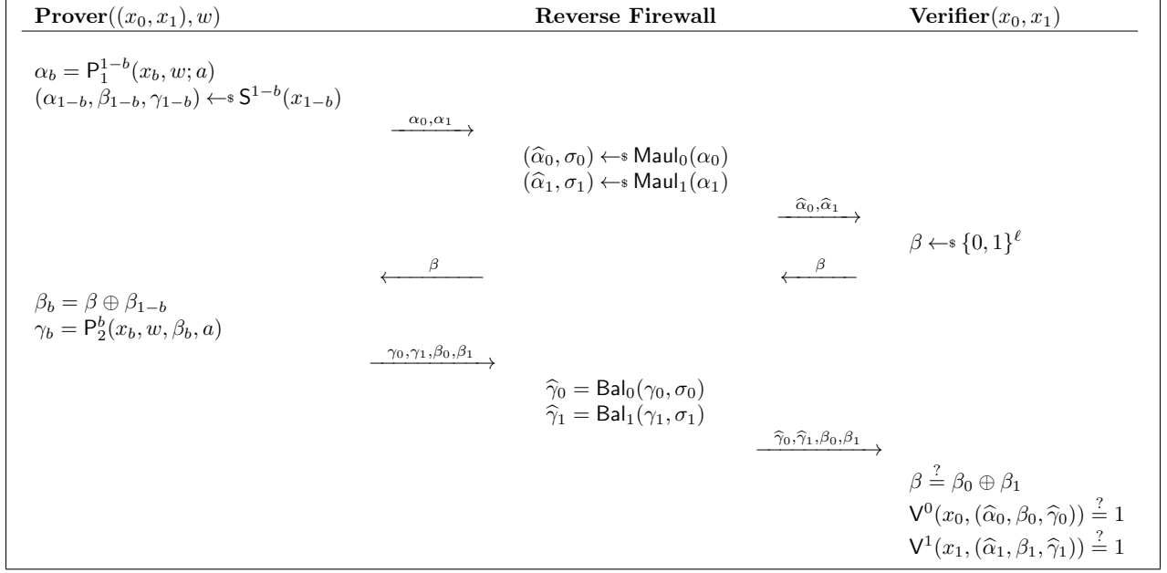
Figure 7: Reverse Firewall for the basic OR composition of Sigma protocols, where b \in \{0, 1\} is s.t. (x_b, w) \in \mathcal{R}_b .
