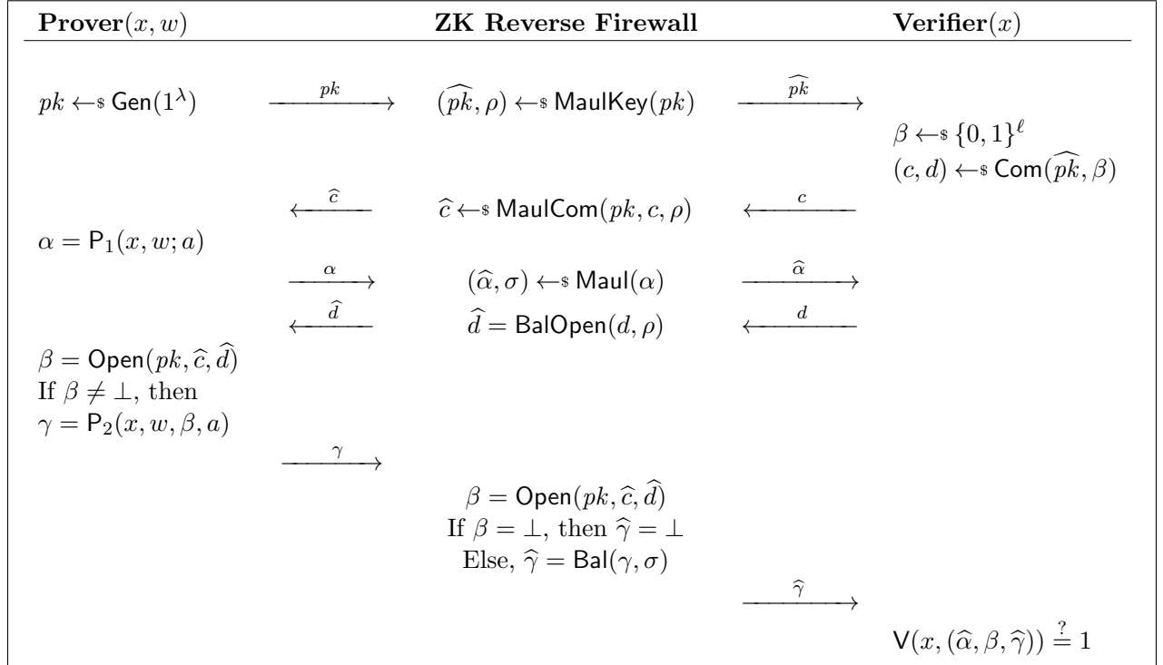
Figure 4: Prover's RF for the protocol in Fig. 3
