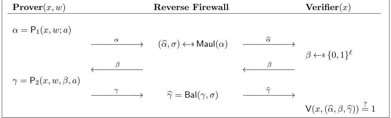
Figure 2: Cryptographic reverse firewall for a malleable Sigma protocol
