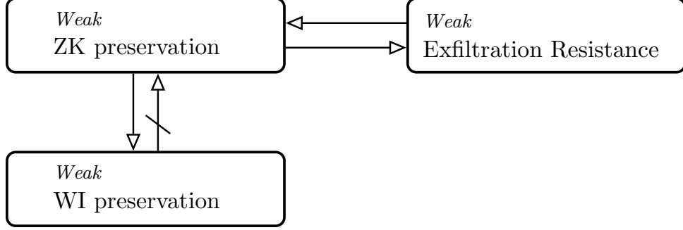
Figure 1: Diagram of relations among the (possible) security definitions for the prover’s RF. We use A \rightarrow B to denote an implication from notion A to notion B , and A \dashrightarrow B to denote a separation from notion A to notion B .
