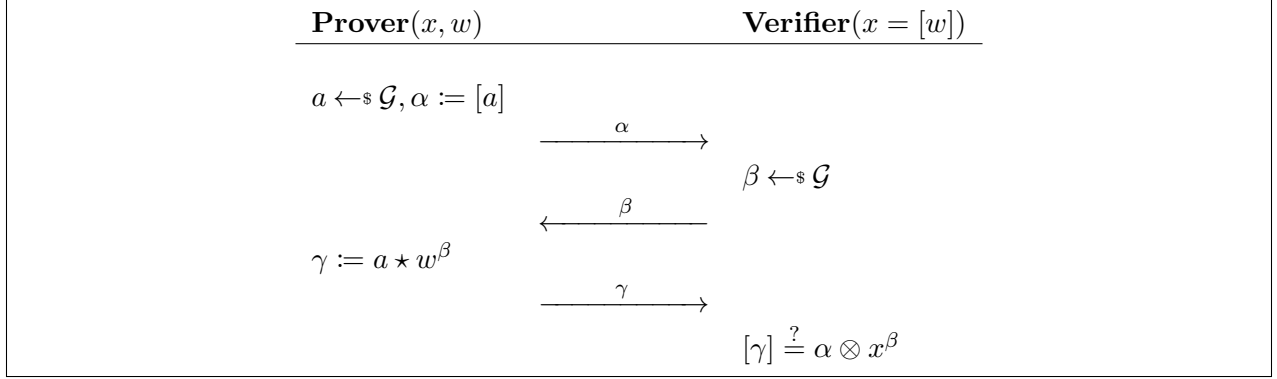
Figure 8: Pre-image protocol for proving knowledge of w such that x = [w]
