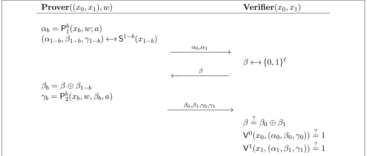
Figure 6: OR composition of Sigma protocols, where b \in \{0, 1\} is s.t. (x_b, w) \in \mathcal{R}_b .
