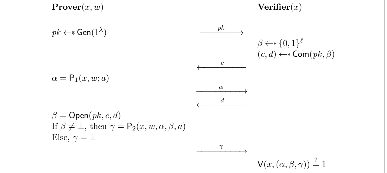
Figure 3: Sigma protocol compiled with standard techniques to obtain full zero knowledge
