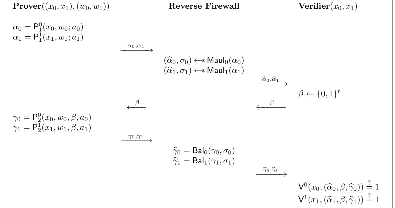
Figure 5: Reverse firewall for the AND composition of Sigma protocols
