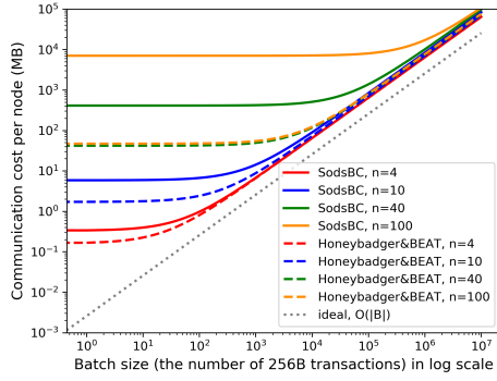
Figure 6: SodsBC Communication Overhead
