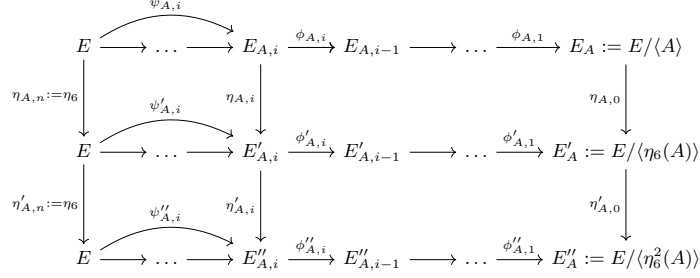
Fig. 2. Isogeny paths between the relevant curves.
