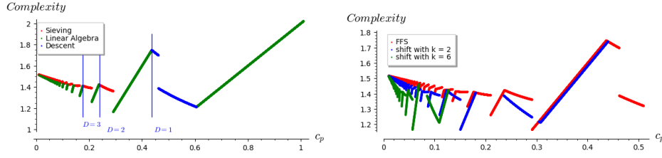
Fig. 3: On the left, the complexity of FFS at the boundary case and the dominant phase as a function of c_p , obtained after fixing the error in [33]. On the right, assuming n has appropriate factors, the lowered complexity of FFS for small values of c_p when considering shifts. In this plot, we consider \kappa = 2, 6 . We only plot points of the curves \mathcal{C}_2 and \mathcal{C}_6 which are lower than the original FFS curve.
