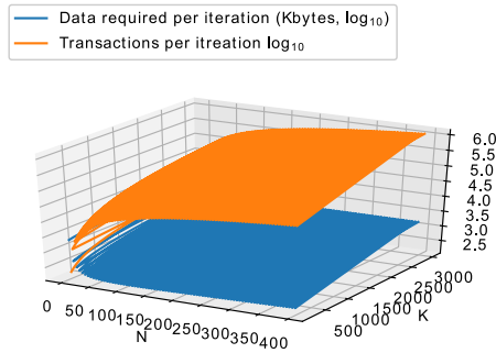
Figure 21: Data requirement and Throughput per iteration with different K and NC when n = 8000 .
