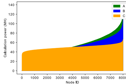
Figure 23: Power distribution
