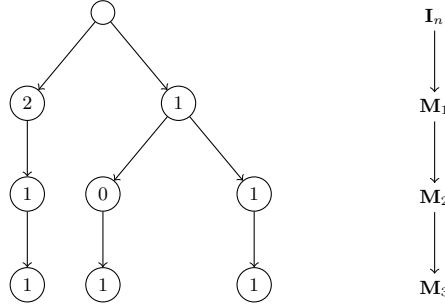
Fig. 2. Example of the tree we obtain for \mathbf{w}_1 = (2, 1, 1) , \mathbf{w}_2 = (1, 0, 1) , \mathbf{w}_3 = (1, 1, 1) . The matrix \mathbf{M}_1 has an eigenspace of dimension 1 E_{1,2} and one of dimension 2 E_{1,1} . At the first iteration we obtain therefore \mathbf{w}_1 . Then we compute the restriction of \mathbf{M}_2 to E_{1,1} ; this has two distinct eigenvalues 0 and 1, which enables to recover the eigenvectors \mathbf{w}_2 and \mathbf{w}_3 . All the nodes at depth 2 represent dimension one spaces, hence the algorithm terminates.
