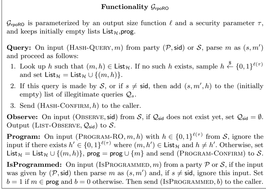
Fig. 13. Restricted observable and programmable global random oracle functionality \mathcal{G}_{\text{rpoRO}} from [13].
