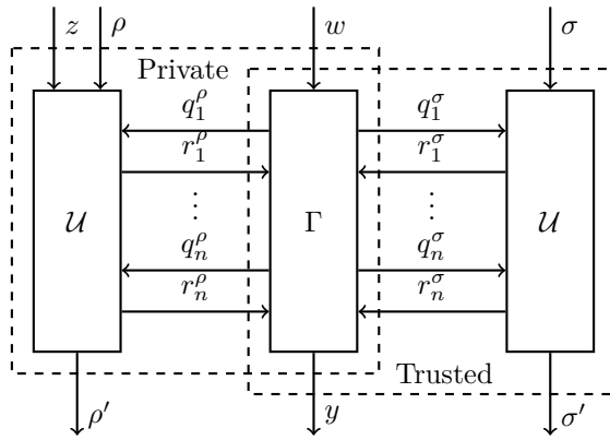
Fig. 4. The interaction of the core contract \Gamma , with two universal machines \mathcal{U} , acting as state oracles over the public state \sigma , and the private state \rho , together with the context z .
