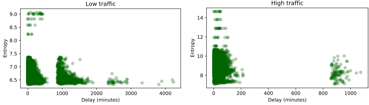
Fig. 9: The sender anonymity (i.e., entropy) in function of the delay for report hashes to arrive at the MS. On the left: 06-01-2020 until 08-01-2020 (summer, low traffic volumes). On the right: 01-11-2020 until 10-01-2021 (winter, high traffic volumes)
