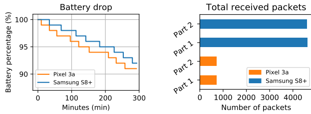
Fig. 13: Battery drop and total received packets for a session of exchange with a switching rate of 30s for the pixel 3a and 3min for the Samsung S8+.
