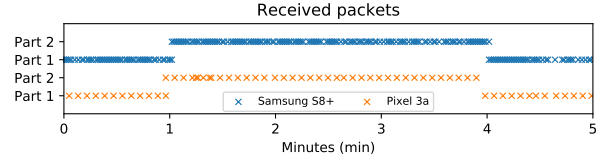
Fig. 12: Advertising and scanning within a time window of 5 min with a common switching rate of 3 min.
