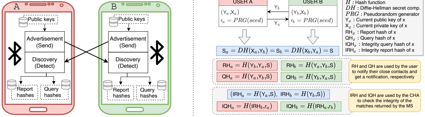
Fig. 3: Close contact registration. All the parameters are intended for the current period t (e.g., X_a , Y_a , and S respectively refer to X_{a,t} , Y_{a,t} , and S_t , and so on). In practice, public and private keys rotate frequently as well as the random number r
