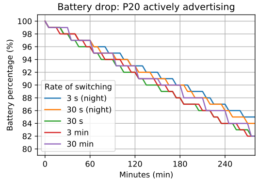
Fig. 11: Battery drop across five experiments.
