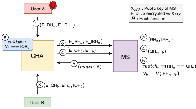
Fig. 6: Integrity check of matches returned by the MS. Step 1 and 2 represent the infection registration phase. Step 3 and 4 are an exposure score request. Along with the matching result, the MS sends an hash which allows the CHA to check whether matches are real. Note that this is a simplified scheme: in practice, the CHA sends batches of encrypted hashes to avoid linkage (Steps 2 and 4).
