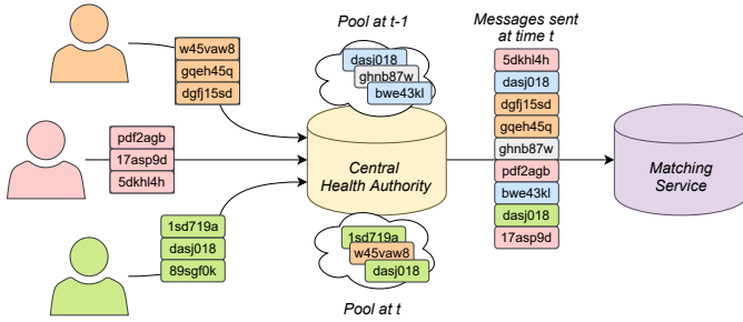
Fig. 7: Batching procedure of the CHA. The CHA collects hashes sent between time t - 1 and t , when a certain condition is met at time t , the CHA shuffles them and sends them in one batch to the matching service.
