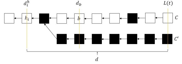
Figure 7: Chains C and C' for an arbitrary attack \pi . In this example, k = 6 , H = 6 , and, A = 9 . d_b - d_i^h = 3 , and, the attack succeeds at time t , at which b is exactly 6 blocks deep in the chain C . Hence, in this example, d is exactly equal to (k-1) + (d_b - d_i^h) = 5 + 3 = 8
