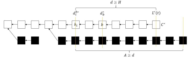
Figure 8: C^* and the private adversary chain under \pi_{SZ} imposed on the same mining times as in Figure 7. Again, k = 6 , H = 6 , and, A = 9 . Adversary has a private chain at depth A + d_i^{h*} = 9 + d_i^{h*} > (k-1) + d_b^* = 5 + d_b^* at time t . Note that at time t , b is not k = 6 blocks deep yet. However, the attack will succeed after b is 6 blocks deep in the chain C^* since the adversary already has a chain that is at depth greater than d_b^* + (k-1) = d_b^* + 5 .
