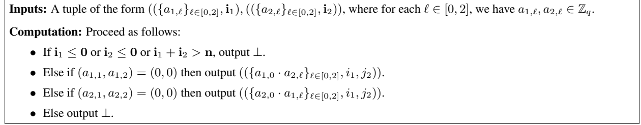
Figure 18: Circuit C_{\text{Mult}, \text{FHE}}
