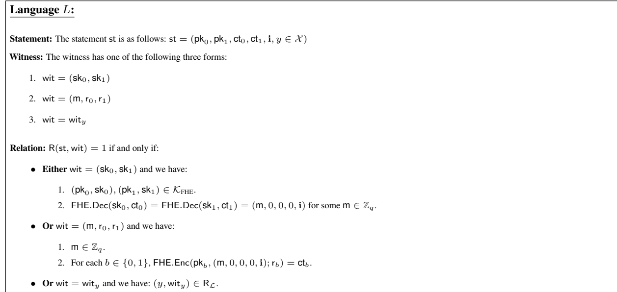
Figure 1: Let \mathcal{K}_{\text{FHE}} be the set of all valid key pairs under the FHE scheme. We define an NP language L as in the figure above. For simplicity, L parameterized by N – the number of levels for our MMap scheme.
