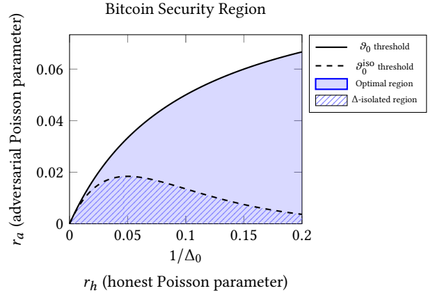
Figure 1: The region of pairs (r_a, r_h) for which Bitcoin is secure with \Delta_0 = 10 . The optimal bound established in this paper \vartheta_0 = 1/(\Delta_0 + 1/r_h) is shown in solid black; the region beneath this line—filled in light blue—is the region of pairs (r_a, r_h) for which we establish security. The best prior bound \vartheta_0^{\text{iso}} = r_h \exp(-2\Delta_0 r_h) is shown in dashed black; its corresponding region of security is shown with blue hatching.
