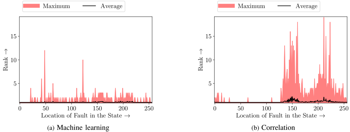
Fig. 5: Performances for machine learning and correlation based methods on GRAIN-128A (with authentication)
