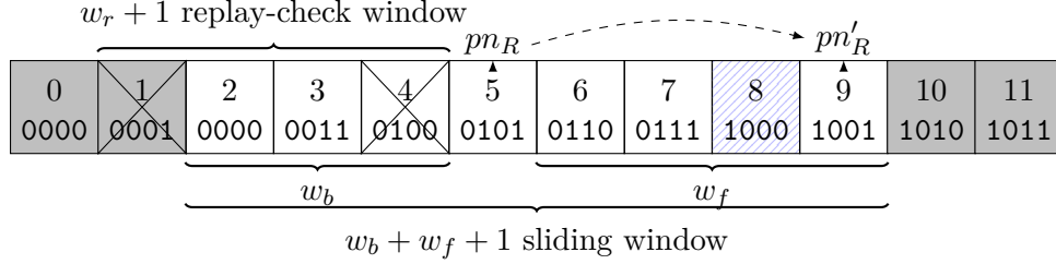
Figure 11: Exemplary illustration of a dynamic sliding receiving window of (toy) size 2^n = 8 (i.e., w_b = 3 and w_f = 4 ) around the next expected packet number pn_R = 5 = 0101_2 , replay-check window of size w_r + 1 = 4 . Packet numbers 1 and 4 have been received before, crossed-out in the replay-window. Grayed-out packet numbers are outside the current sliding window.
