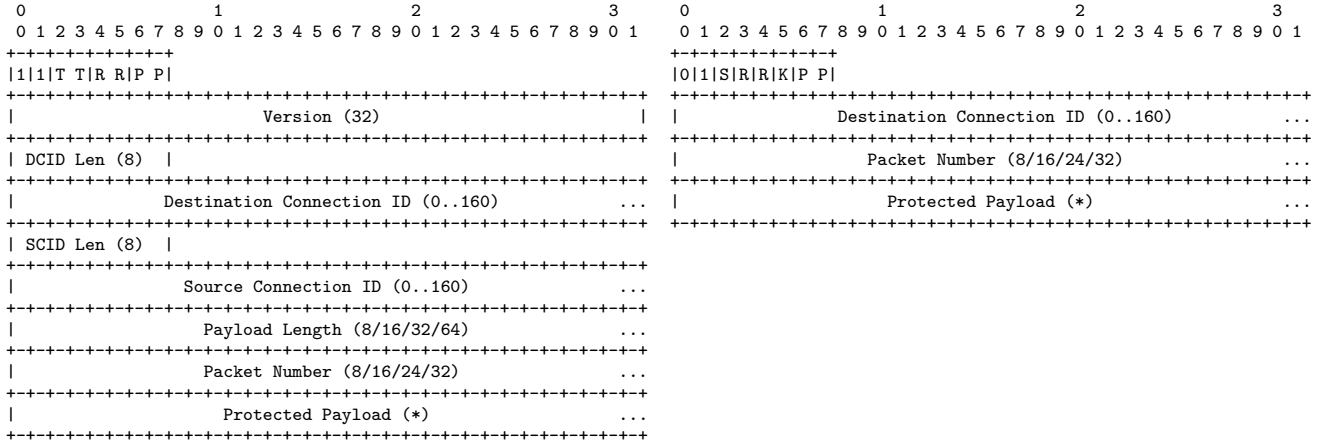
Figure 9: QUIC packet formats for long (left) and short (right) packets [IT21, Section 17]. The first byte contains flags T: Type, R: Reserved, P: Packet number length, S: Spin, K: Key phase. Field bit-length is given in parentheses, (*) indicating variable length.
