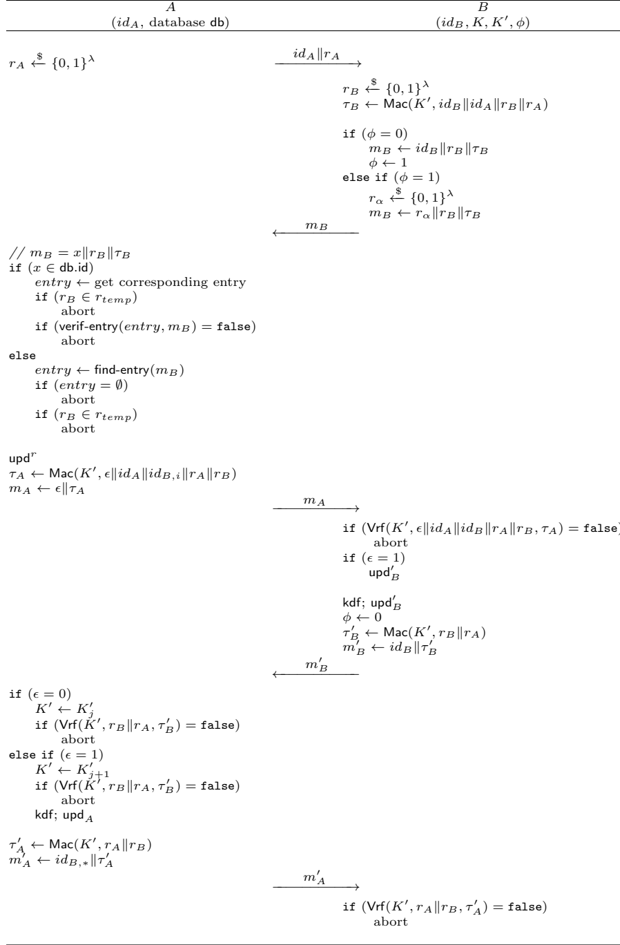
Fig. 3: The SAKE + and SAKE + -AM protocols (based on our understanding of [1], Section 6.2 and Figure 2)
