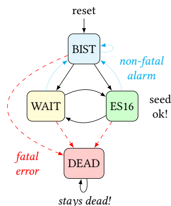
Figure 2: Normally the operational state alternates between WAIT (no data) and ES16, which means that 16 bits of randomness (seed) has been polled. BIST (Built-in Self-Test) only occurs after reset or to signal a non-fatal self-test alarm (if reached after WAIT or ES16). DEAD is an unrecoverable error state.
