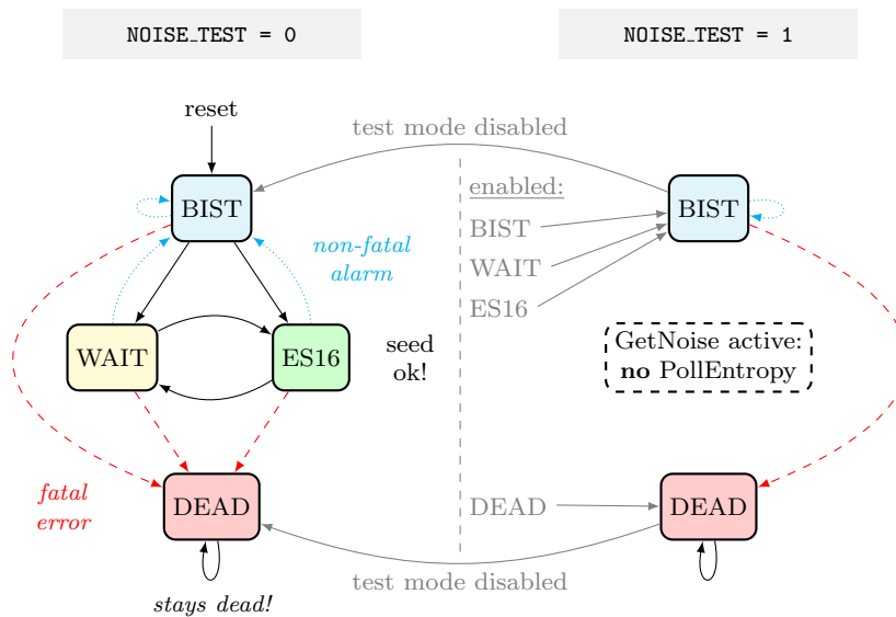
Fig. 2 Normally the operational state alternates between WAIT (no data) and ES16 , which means that 16 bits of randomness (seed) has been polled. BIST (Built-in Self-Test) only occurs after reset or to signal a non-fatal self-test alarm (if reached after WAIT or ES16 ). DEAD is an unrecoverable error state. In test mode (when GetNoise is active) WAIT and ES16 states are unavailable in PollEntropy .
