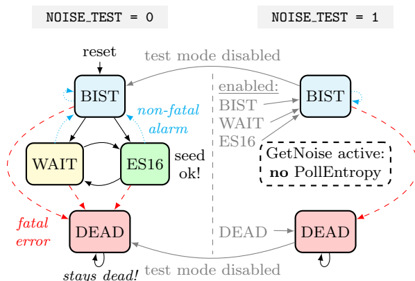
Fig. 2 Normally the operational state alternates between WAIT (no data) and ES16 , which means that 16 bits of randomness (seed) has been polled. BIST (Built-in Self-Test) only occurs after reset or to signal a non-fatal self-test alarm (if reached after WAIT or ES16 ). DEAD is an unrecoverable error state. In test mode (when GetNoise is active) WAIT and ES16 states are unavailable in PollEntropy .
