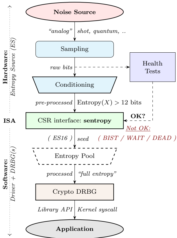
Fig. 1 The sentropy CSR provides an Entropy Source (ES) only, not a stateful random number generator. As a result, it can support arbitrary security levels. Cryptographic (AES, SHA-2/3) ISA Extension instructions can be used to construct high-speed DRBGs that are seeded from the entropy source.
