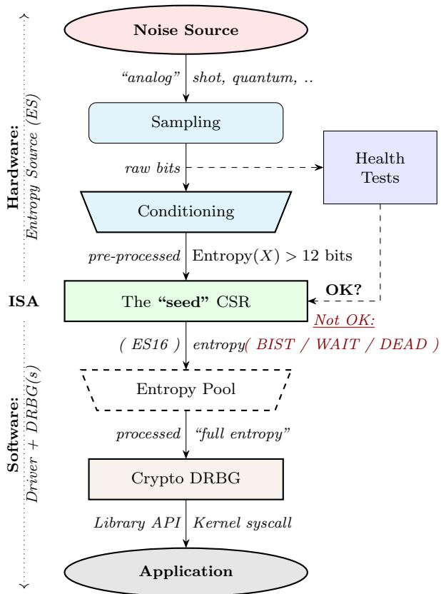
Fig. 1 The seed CSR provides an Entropy Source (ES) only, not a stateful random number generator. As a result, it can support arbitrary security levels. Cryptographic (AES, SHA-2/3) ISA Extension instructions can be used to construct high-speed DRBGs that are seeded from the entropy source.
